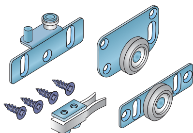
Sada S27AL/S37AL
